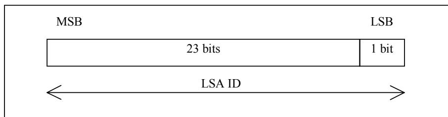
Figure 19: Structure of LSA ID
