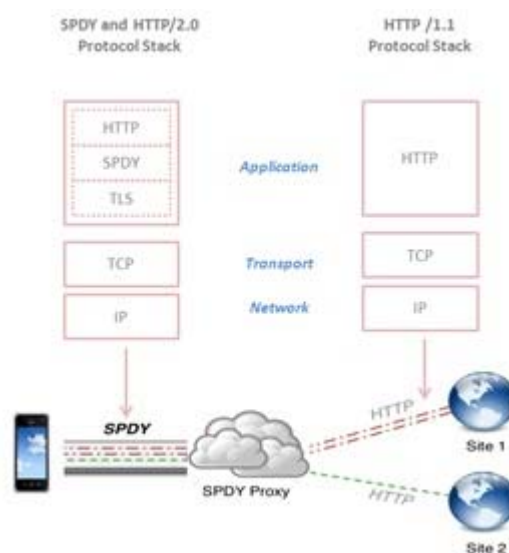
Figure 4: The SPDY/HTTP/2.0 and HTTP/1.1 protocols
